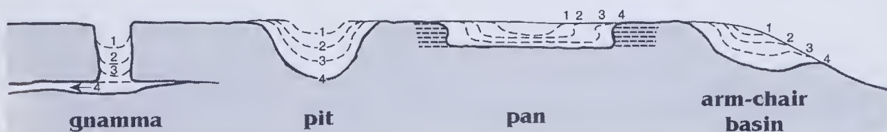
Figure 5. Schematic showing the development of gnammas, pits, pans and arm-chair basins by progressive weathering, indicated by numbers (drawn from Campbell 1997).
